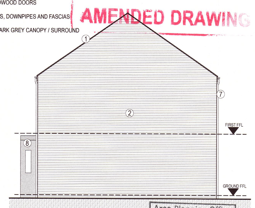
LEFT SIDE ELEVATION BLOCK A
